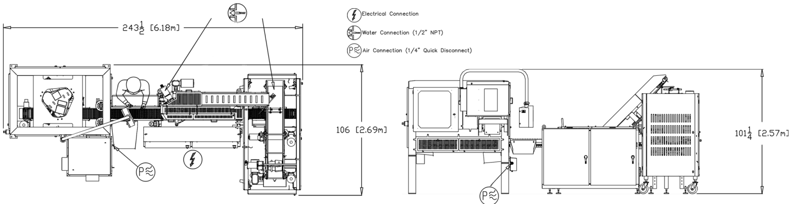
Configuration is 90 degrees. Packaging machine is not shown.
